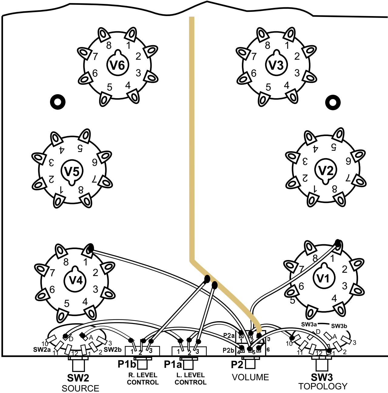
WIRING DIAGRAM 4B (dual outputs)
