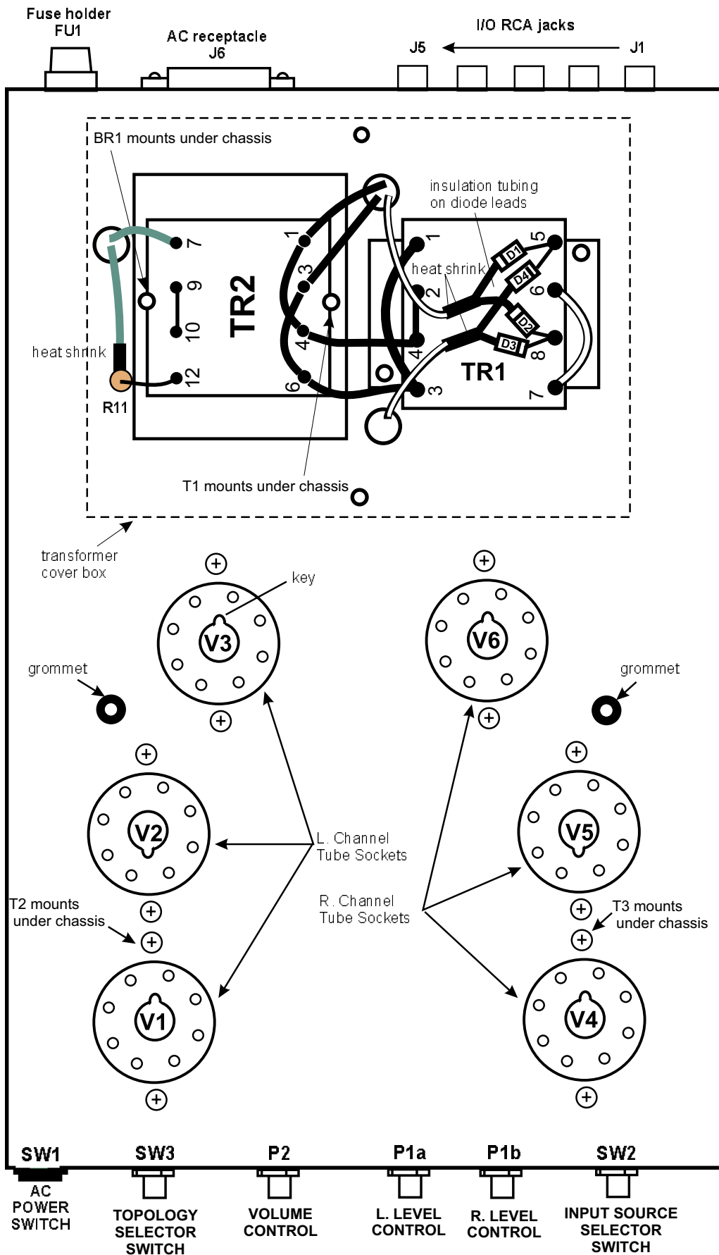
WIRING DIAGRAM 1 (top of chassis)
