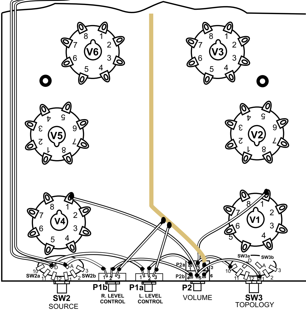
WIRING DIAGRAM 4A (record output)
