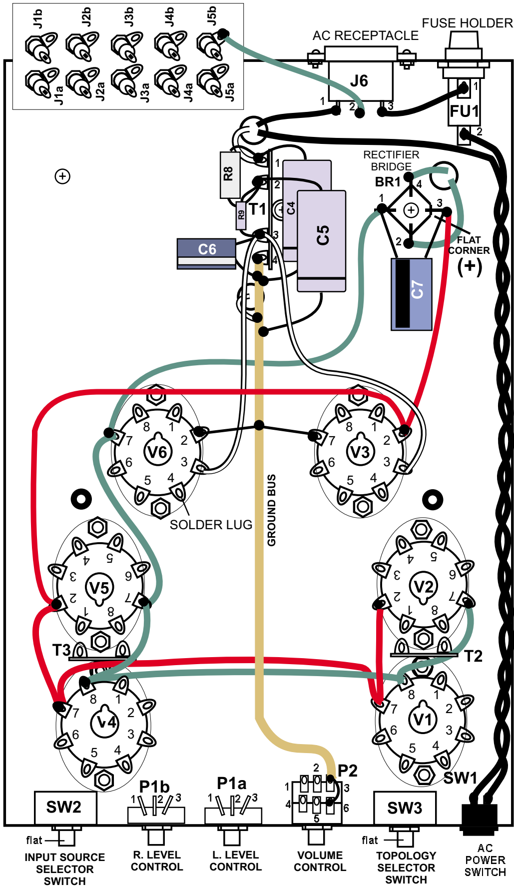
WIRING DIAGRAM 2 (underside of chassis)
