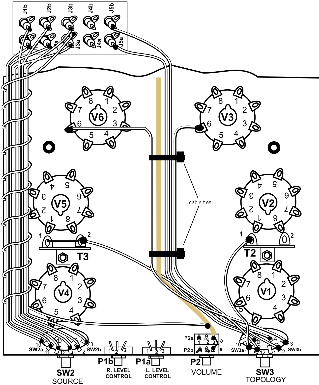
WIRING DIAGRAM 5
