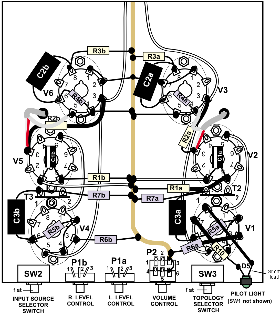
WIRING DIAGRAM 3 (underside of chassis)
